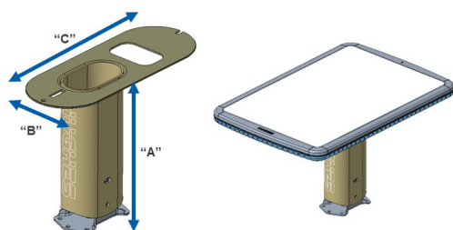
(3) Penetrating Mount with Tall Stanchion
