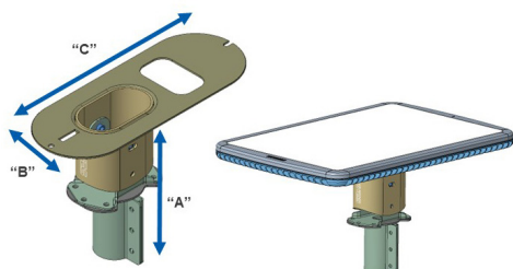
(1) Mast Adapter Mount (Mates to 2-3/8 inch OD Pole)
